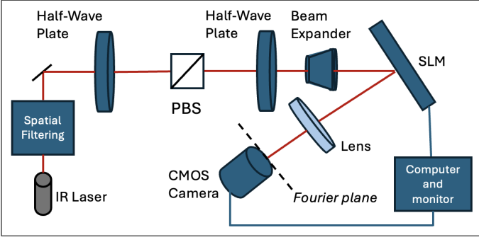
Figure 6: Schematic of the experimental setup for the JTC-based optical correlator. The laser beam is expanded and collimated, modulated by the SLM, and Fourier-transformed onto the CMOS camera.
